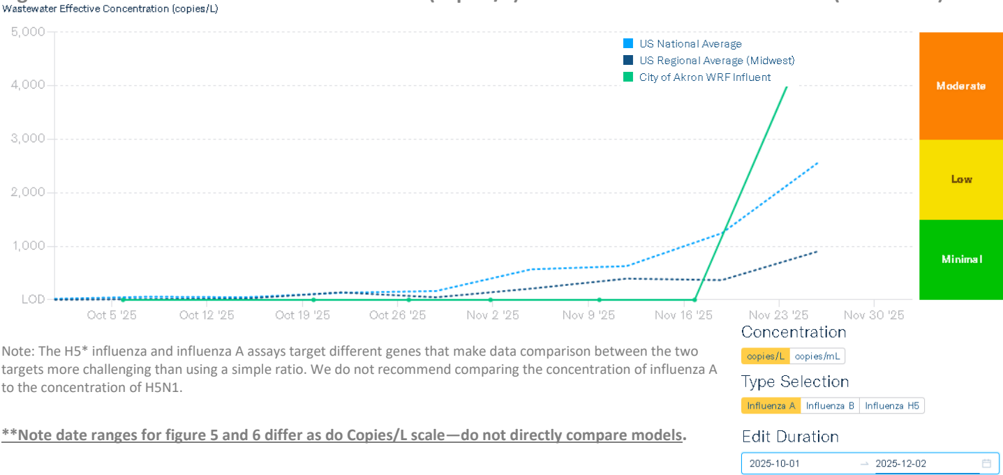
Figure 5. Wastewater Effective Concentration (copies/L) of Influenza A for current season (2025-2026):
