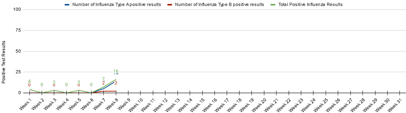
Figure 4. Influenza diagnostic tests with positive results completed by Summit County health facilities, 2025 to 2026 season
